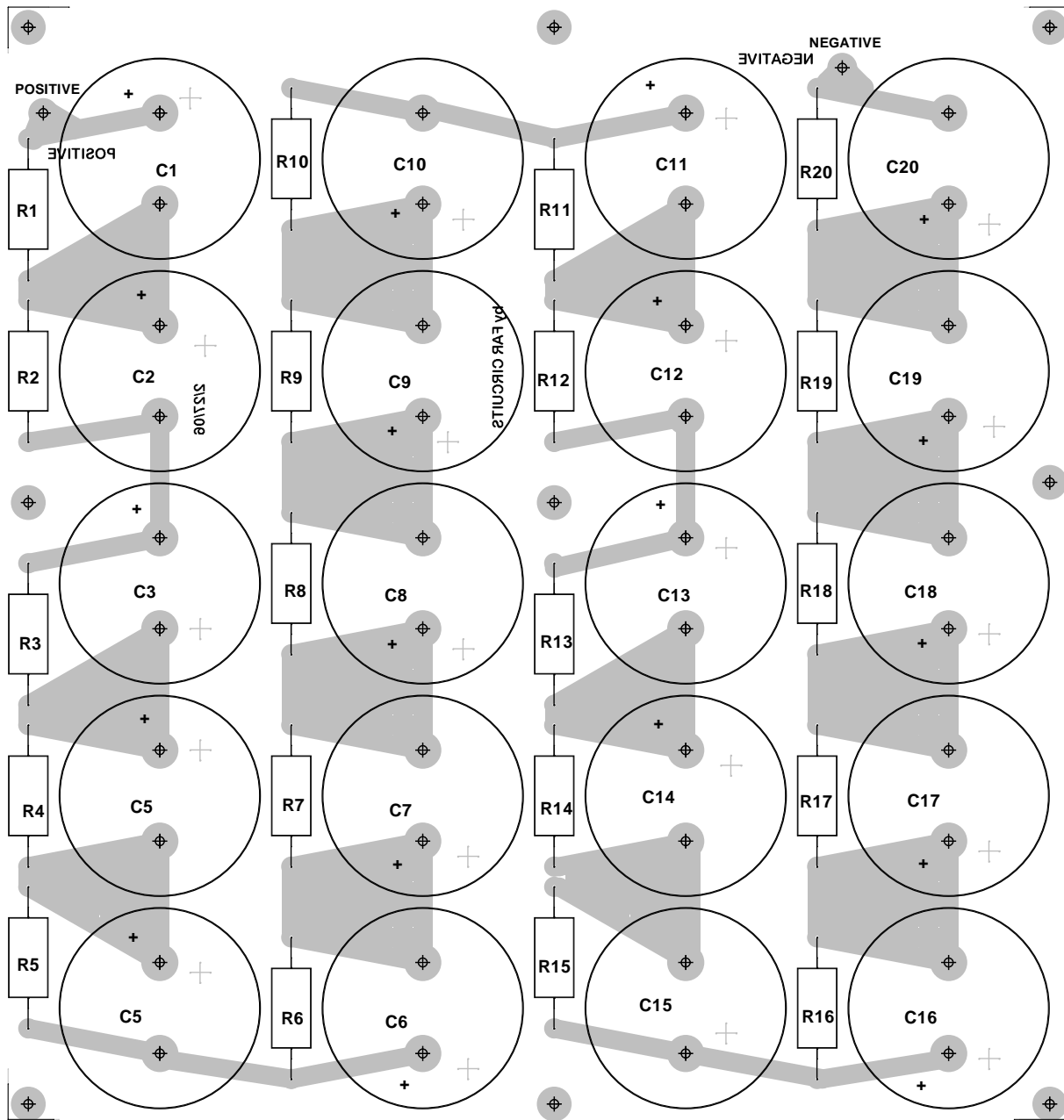
RESISTORS ARE 3 W METAL FILM 100K CAPACITORS ARE 1500uf AT 450 WVDC 10.5" BY 11.00"
