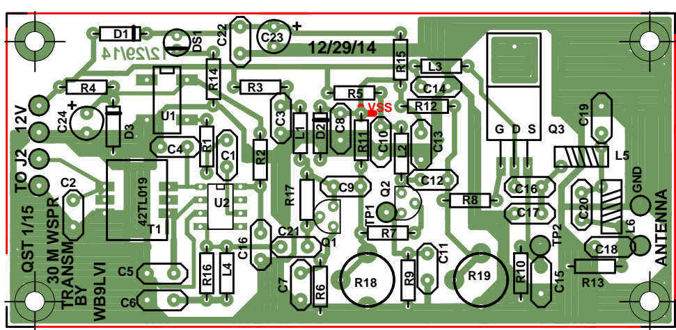
30 METER WSPR TRANSMITTER QST JAN 2015 $7.00
